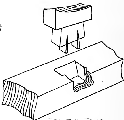
FOX-TAIL TENON
